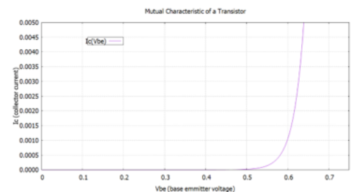
Gambar 1. Mutual characteristic of transistor
